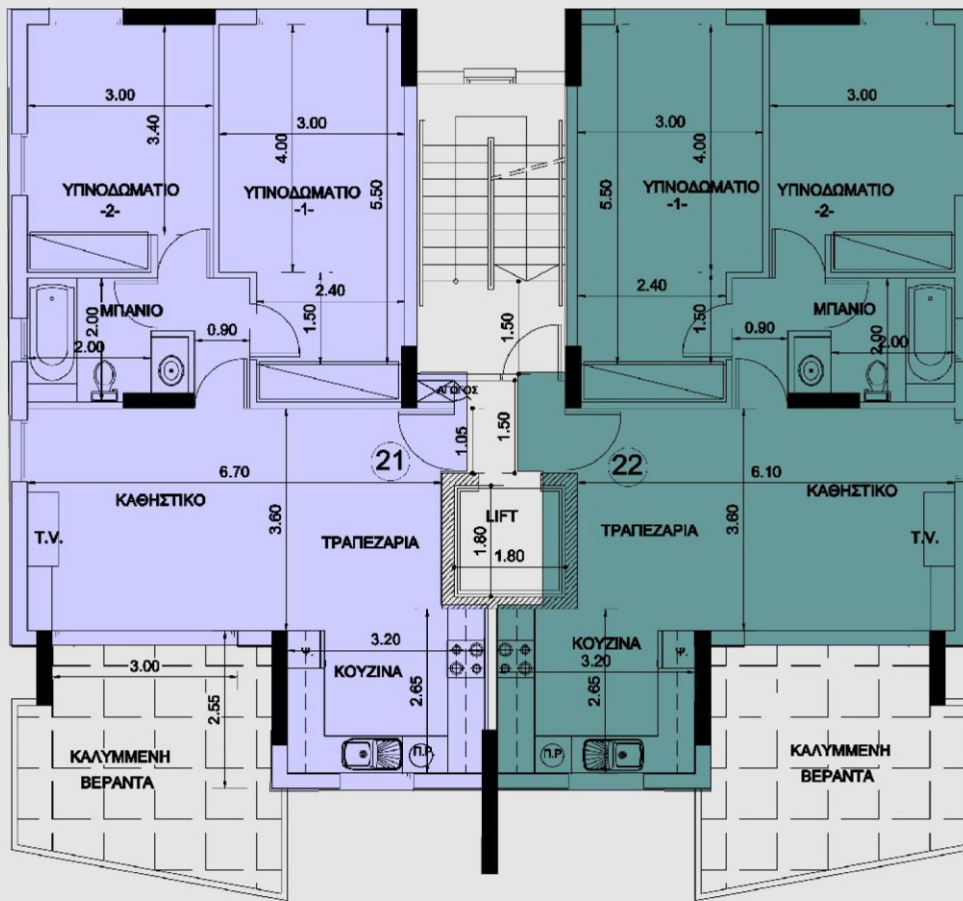
TYPICAL FLOOR
